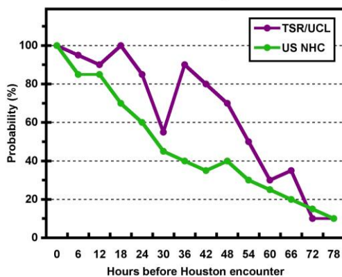
Chance of Hurricane Ike striking Houston with hurricane-strength winds
